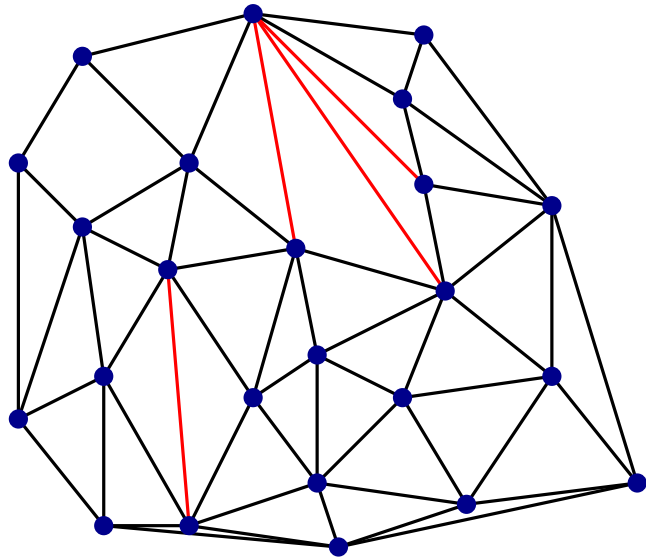
non-Delaunay triangulation
