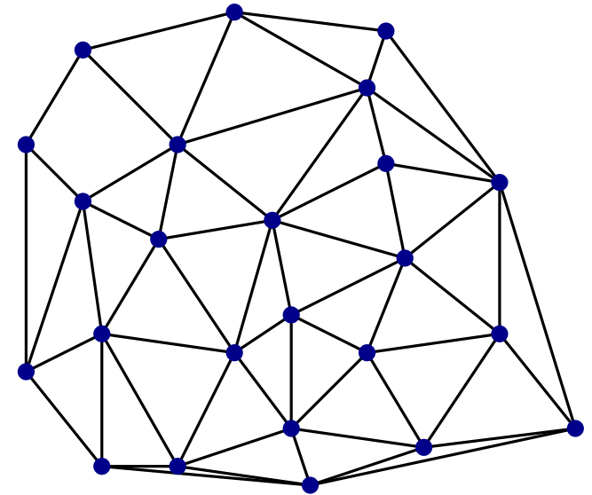
Delaunay triangulation
